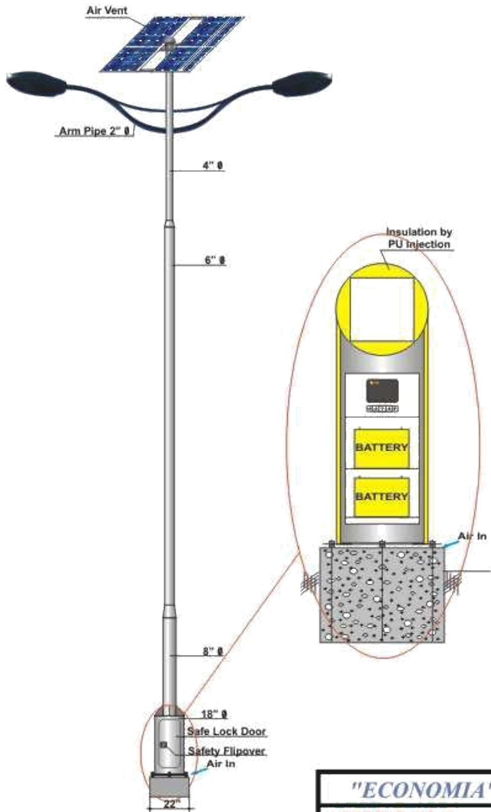
DETAIL STRUCTURE DESIGN OF ECONOMIA DOUBLE ARM SOLAR STREET LIGHT
